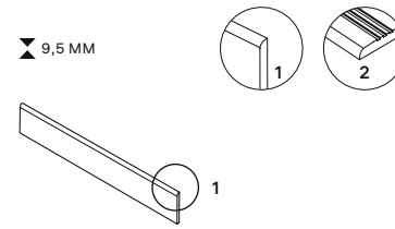
skirting plinthe sockel rodapé boleado 8x89 . 3,2"x35" P MP-6270 8x90 . 3,2"x36" SM MP-6260 8x120 . 3,2"x48" SM MP-6260 P MP-6270
