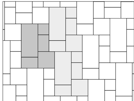
4D 32x32_9,29% . 32x48,1_27,89% . 48,1x48,1_20,94% . 48,1x96,4_41,88% module also available boxed - 1 piece 32x32 nt/crs, 2 pieces 32x48,1 nt/crs, 1 piece 48,1x48,1 nt/crs, 1 piece 48,1x96,4 nt/crs in each box | modulo disponibile anche inscatolato - 1 pz. 32x32 nt/crs, 2 pzz. 32x48,1 nt/crs, 1 pz. 48,1x48,1 nt/crs, 1 pz. 48,1x96,4 nt/crs in ogni scatola
